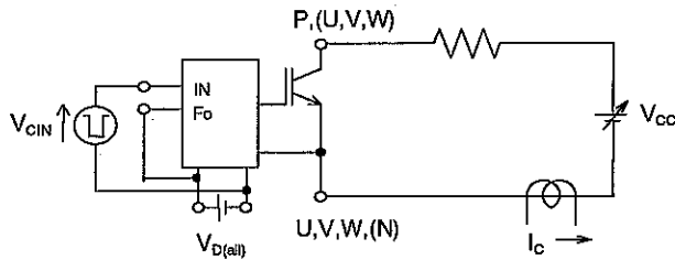
Fig.5 SC Test
